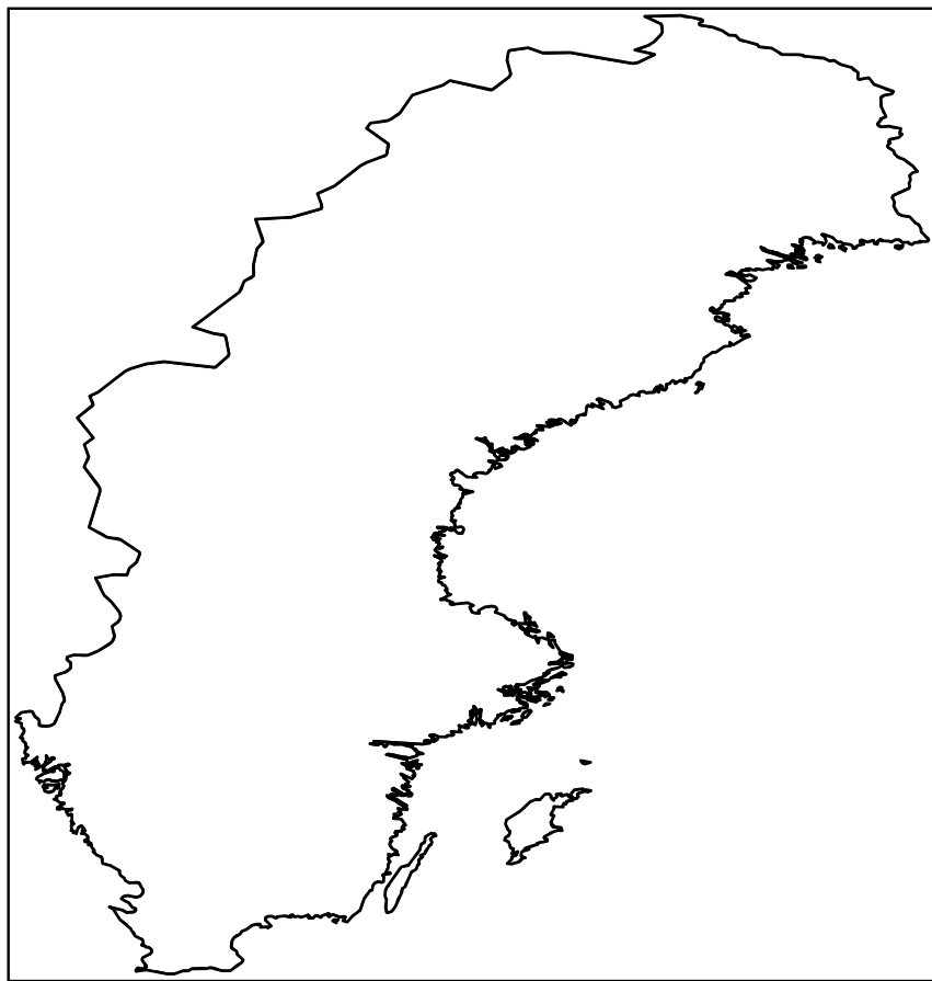
DI12 and spring wheat yield
